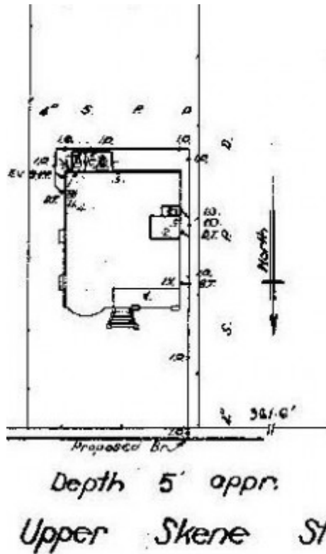
GWST Drainage Plan no. 4713A, 1937, Barwon Water.
